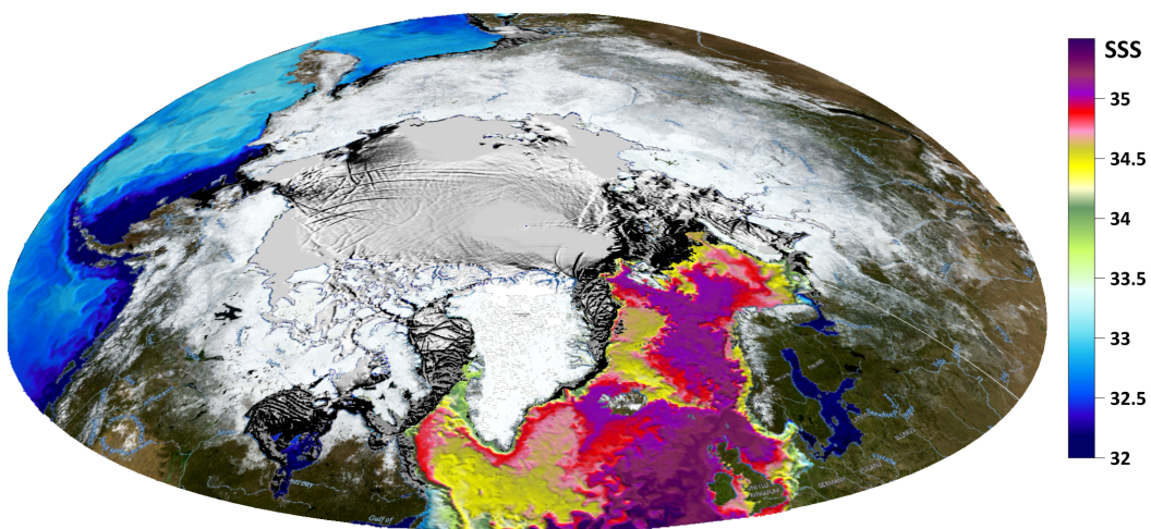
Fig.2 Arctic sea ice compactness and sea surface salinity
